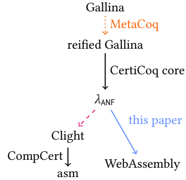
Figure 1. The CertiCoq pipeline. Proofs in progress are in dashed magenta, and MetaCoq [9] (which has to be trusted) is in dotted orange. Our verified contribution is in blue. The CertiCoq core stage includes optimisations on \lambda_{\text{ANF}} .
